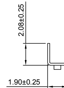
SEC:C-C
