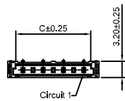
Circuit 1
