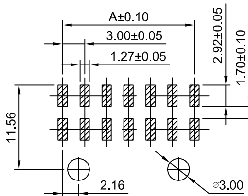
P.C.B LAYOUT (2x4P~2x12P)
