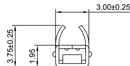
SEC:C-C
