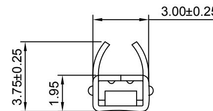
SEC:C-C
