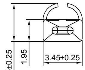
SEC:C-C
