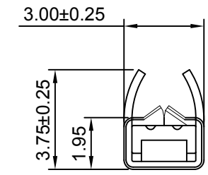
SEC:C-C
