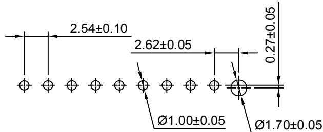
PCB LAYOUT
