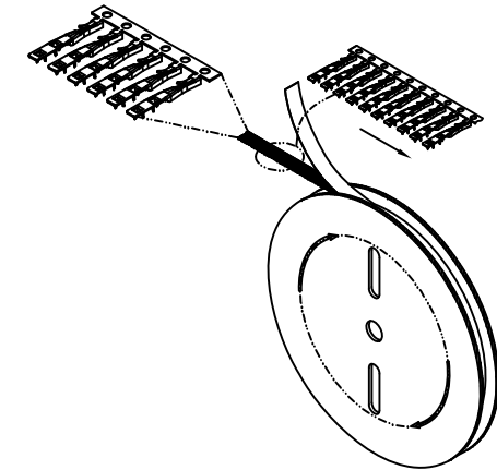
Winding Direction
