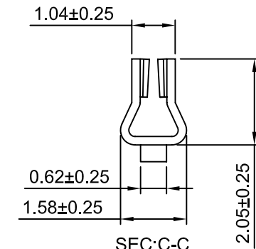
SEC:C-C
